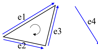
Fig. 1. Incidence of oriented triangles and edges. e_1 is positively incident to the oriented triangle, e_2 and e_3 are negatively incident, and e_4 is not incident to the triangle.
