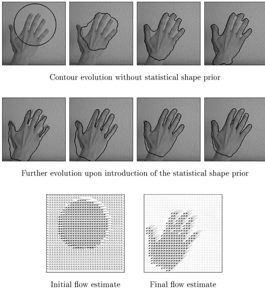
Fig. 5. Effect of the statistical shape prior. The hand is moving to the bottom left. The statistical shape prior is introduced upon stationarity of the contour (middle row). Initial and final estimates of the flow field (bottom) show the improved separation of the two motion fields. The final segmentation is cut at the wrist, because the training shapes were all cut at this location for simplicity.
